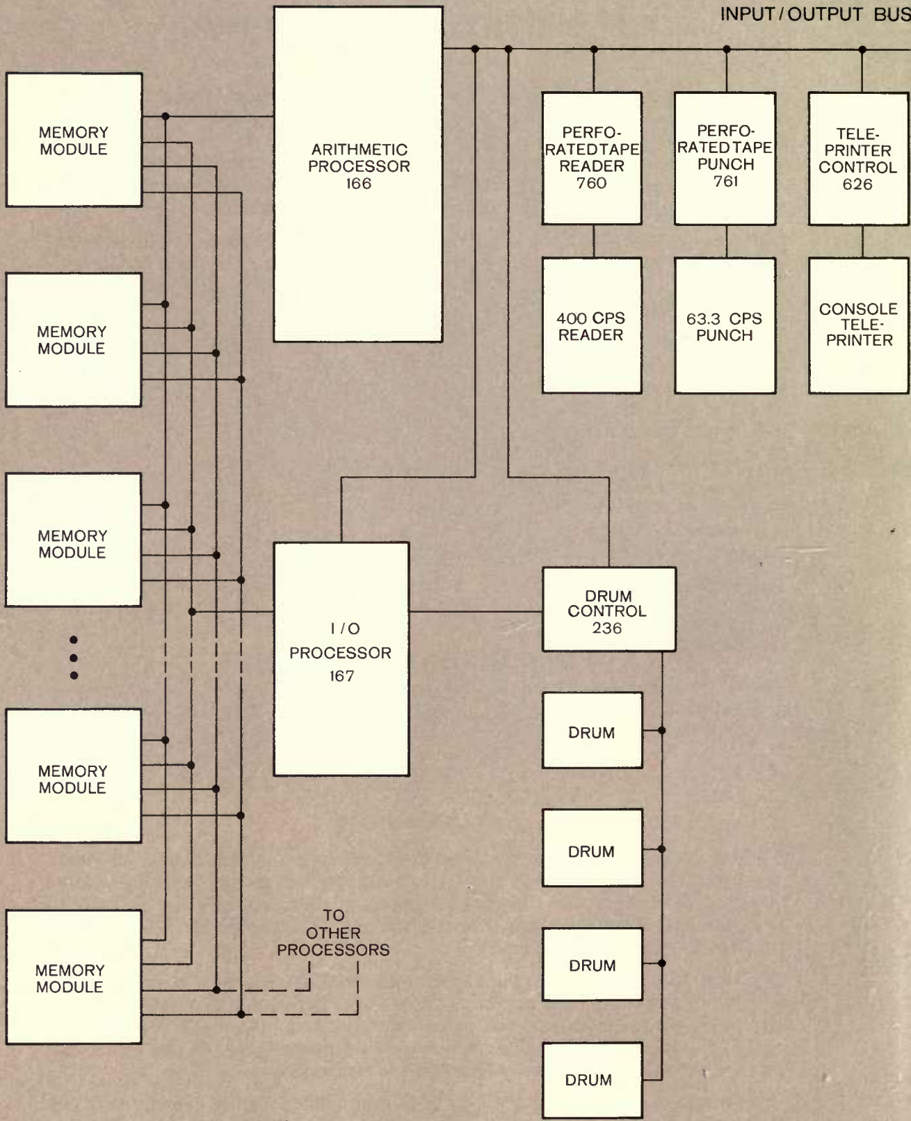
Figure 3 PDP-6 System Interconnections
